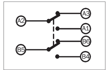
Contact arrangement on Type 9201
