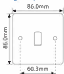
1 Gang Frontplate
