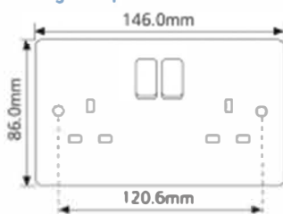
2 Gang Frontplate
